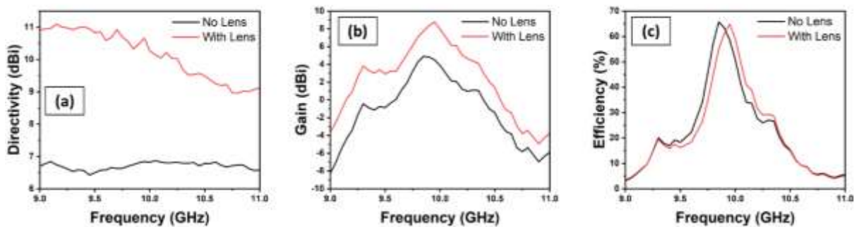
Figure 8 – Measured antenna results (a) Antenna Directivity, (b) Antenna Gain and (c) Total Efficiency of the antenna with/without the 3D printed hemispherical lens.
