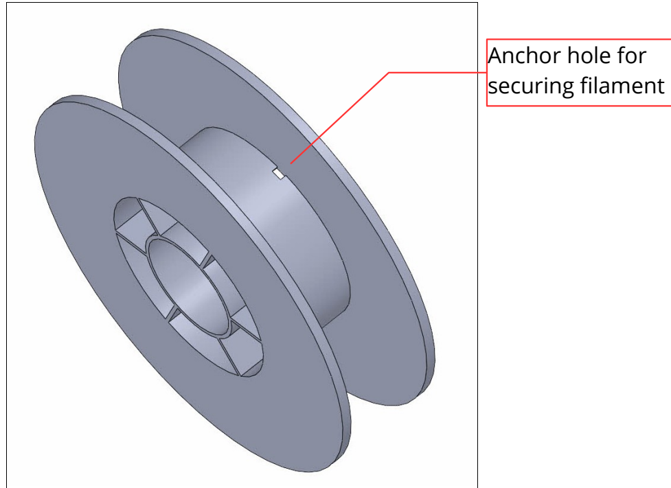
Image 9: Securing filament.
