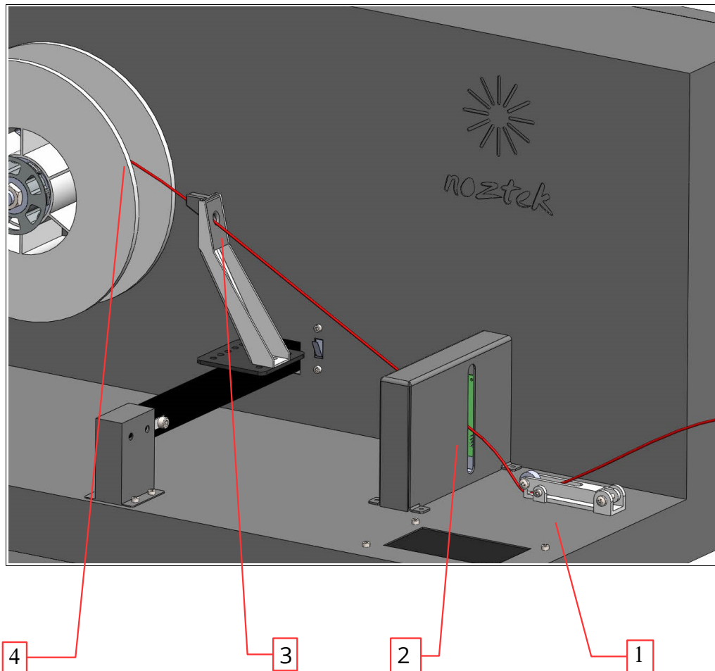
Image 8: Filament loading.
